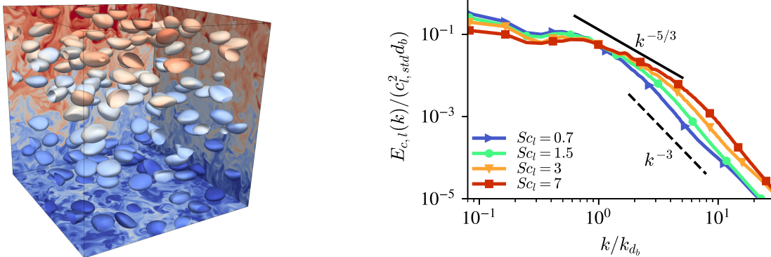
Figure 2: Left panel: Contours of the scalar field in a turbulent bubbly flow with a gas volume fraction \phi = 5.2\% and a mean scalar gradient in the vertical direction. Right panel: Corresponding scalar fluctuation spectra at various liquid Schmidt-numbers Sc_l .
